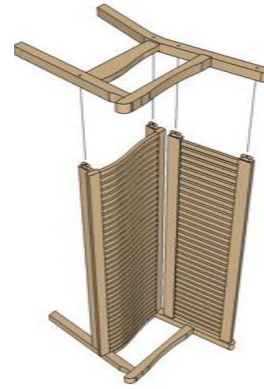
GARDEN BENCH
