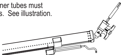
Correct burner-to-valve engagement
